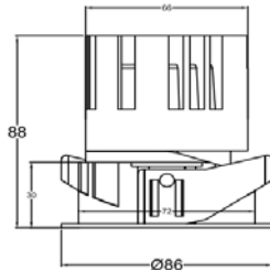
75mm cut-out 10W / 12W
