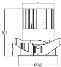
55mm cut-out 10W
