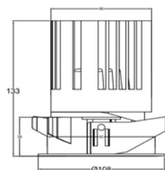
95mm cut-out 18W / 25W / 30W
