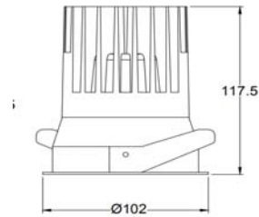
95mm cut-out 18W / 24W
