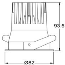
75mm cut-out 10W / 12W / 15W
