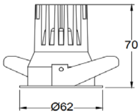
55mm cut-out 7W
